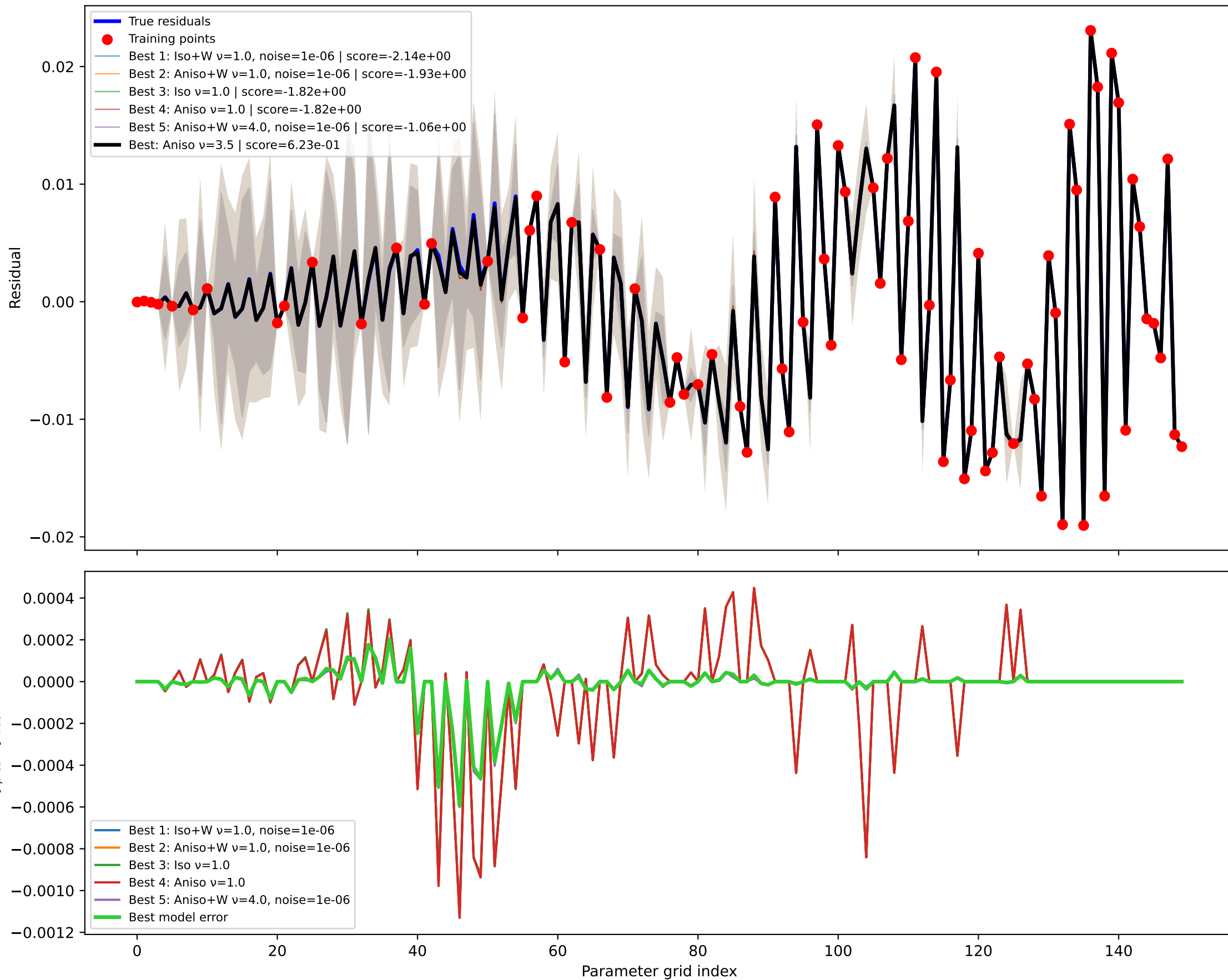
GPR kernel comparison node=11 RMSE=1.006e-04, train RMSE=1.002e-11
